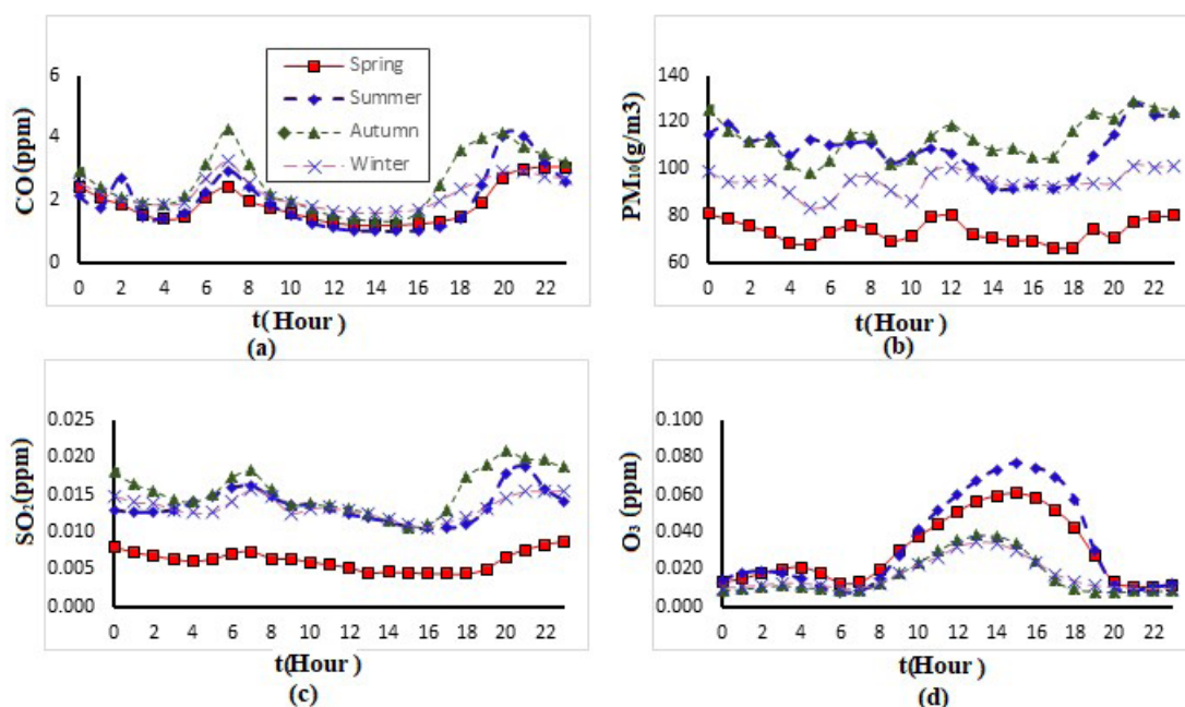
Fig. 4. Recent mean diurnal changes in CO, PM 10 , SO 2 and O 3 pollutants in different seasons in 2016.
