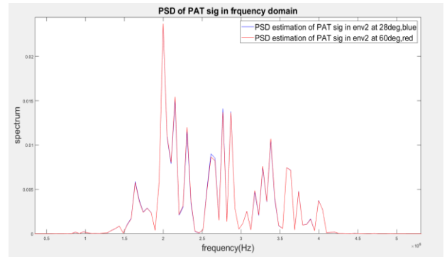
Figure 7. PSD of spectral radiation of two black body in environment2 with a temperature of 28(blue line) and 60 °C (red line) are shown
