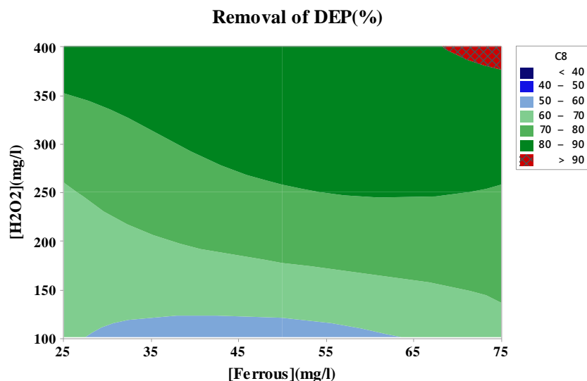
Figure 5) Contour plots of diethyl phthalate removal versus ferrous and hydrogen peroxide concentrations ( pH = 3 ; T = 25^{\circ}C ; t = 60 \text{ min} )
