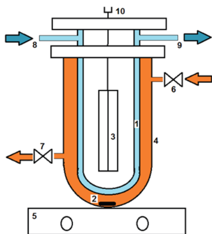
Figure 1) Schematic diagram of used laboratory reactor; (1) cooling water jacket; (2) magnetic stirrer bar; (3) ultraviolet lamp; (4) glass reactor; (5) magnetic stirrers; (6) input wastewater; (7) output wastewater; (8) cooling water input; (9) cooling water output; (10) electric connection
