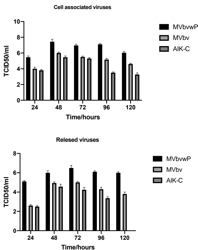
Fig. 5. Growth curve analysis. Vero cells were infected at a MOI of 0.03 PFU of AIK-C, MVbv, or recombinant MVbvwp and incubated at 37 °C. Titration test was done by TCID50 method on cell-associated viruses (A) and cell-free viruses (B) at different time points. The results were represented as the mean of three independent experiments.
