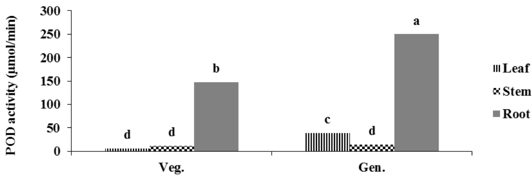
Figure 1. POD activity in the different parts of M. laevigata at both vegetative and generative phases. Vertical bars represent ± S.E. and the same letters are not significantly different at 5% level
