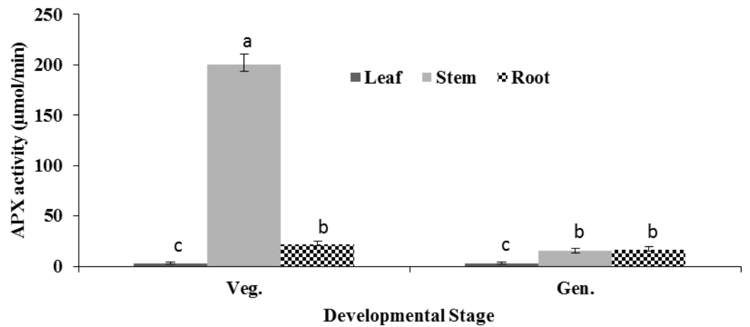
Figure 2. APX activity in the different parts of M. laevigata at both vegetative and generative phases. Vertical bars represent ± S.E. and the same letters are not significantly different at 5% level.
