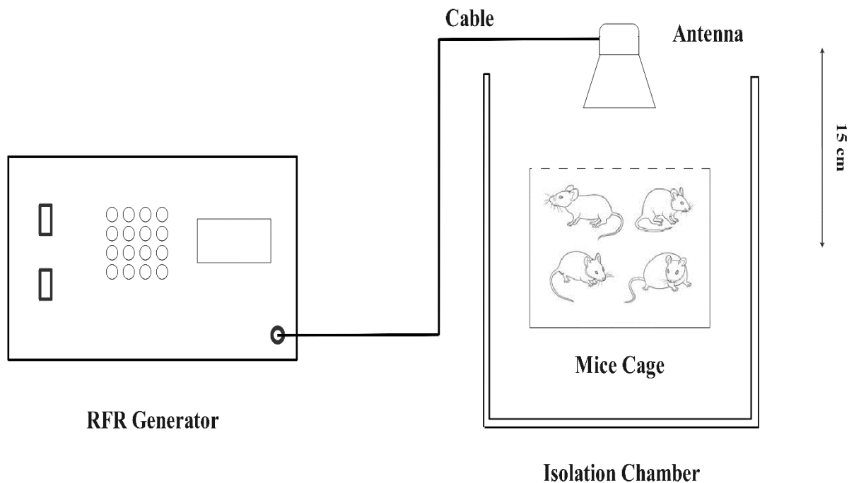
Figure 1: Exposure setup
