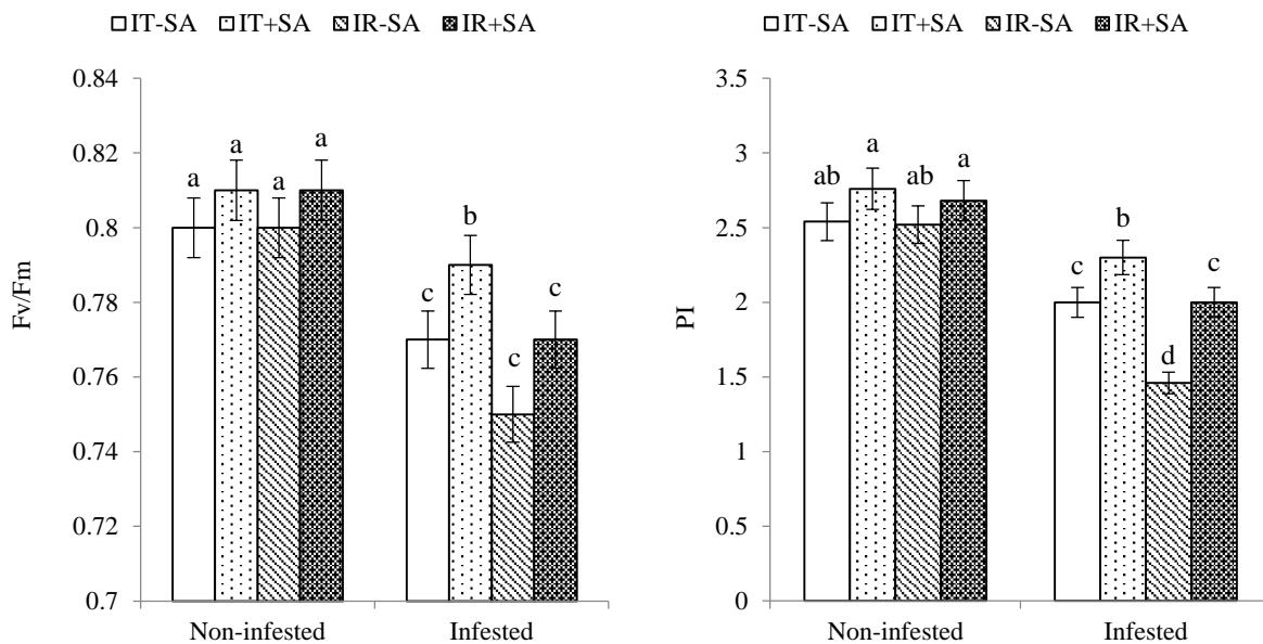
Figure 1. Response of basil varieties to salicylic acid under field dodder infestation; (a): F v /F m ; (b): PI; each value is the mean four replicates; bars represent standard error of the mean; means with different letters within each characteristic show significant difference, based on Duncan's Multiple Range Test at p ≤ 0.05); IT: Italian variety; IR: Iranian variety; SA: salicylic acid.
