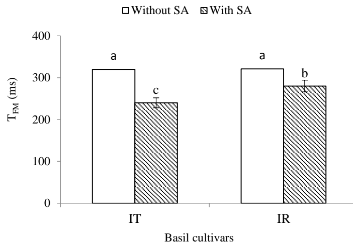
Figure 2. Changes in T_{FM} of basil varieties (left in response to salicylic acid application; each value is the mean of four replicates; means with different letters show significant difference, based on Duncan's Multiple Range Test at p \leq 0.05 ); IT: Italian variety; IR: Iranian variety; SA: salicylic acid.
