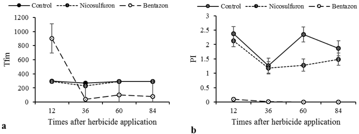
Figure 5. Changes in Tfm (a) and PI (b) of spiny cocklebur ( Xanthium spinosum L.) after 12, 36, 60 and 84 hours of nicosulfuron and bentazon herbicides application.
