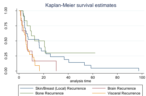
Figure 3. Survival from metastasis until death in recurrence patients. X axis is indicative of weeks and Y axis is the survival rate
