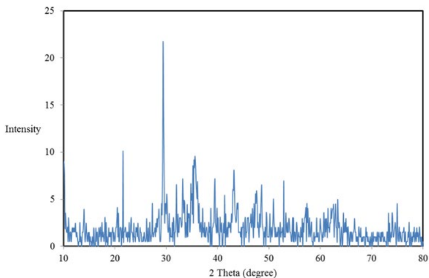
Fig. 3. XRD pattern of Fe 3 O 4 /AC nanocomposite
