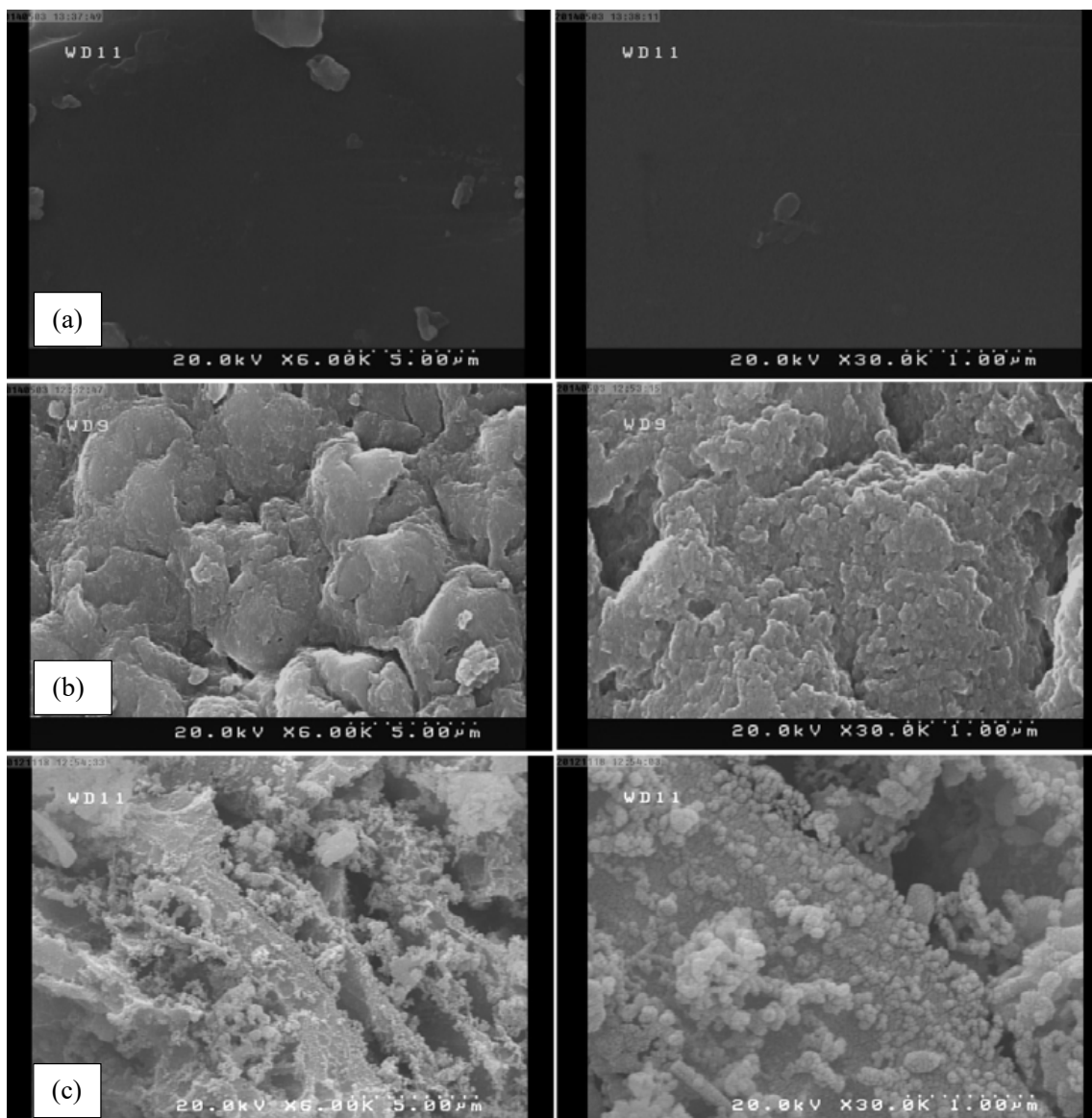
Fig. 2. FESEM image of (a) Raw M (b) activated carbon and (c) \text{Fe}_3\text{O}_4/\text{AC} nanocomposite at different magnification
