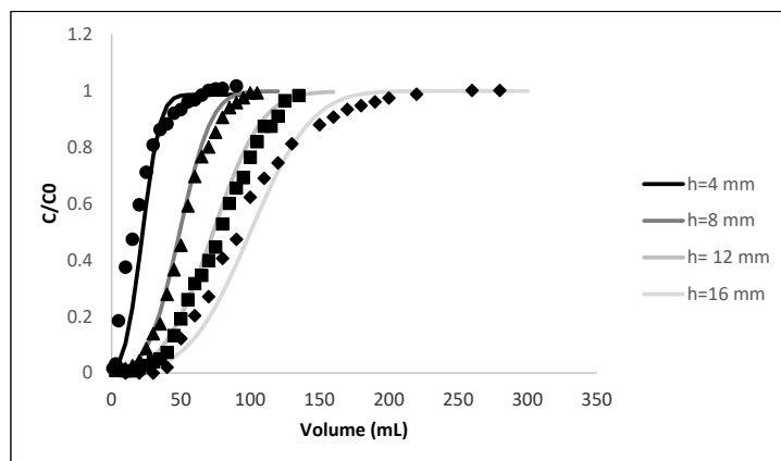
Fig. 4. Effect of bed height on the adsorption of nicotine by AM.
