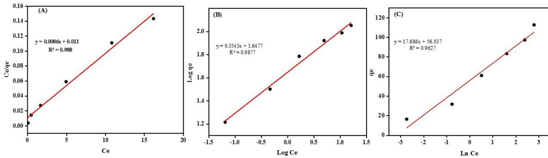
Fig. 5. A) The curve of Langmuir model, B) The curve of Freundlich model and C) The curve of Temkin model of equilibrium isotherm models of 2,4-D adsorption on Fe_3O_4@SiO_2-NH_2 adsorbent
