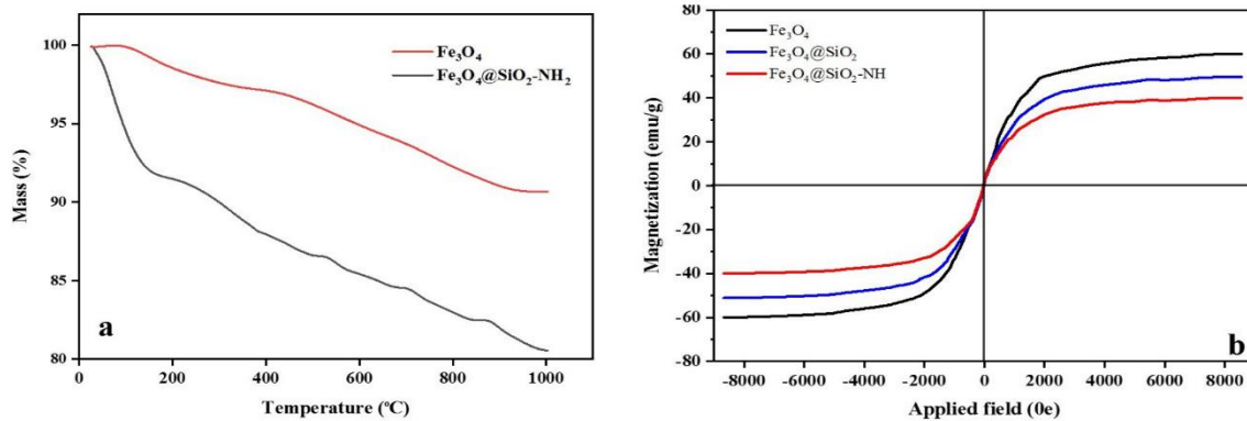
Fig. 3. a) TGA thermal analysis and b) VSM magnetic analysis of synthesized nanoparticles Fe_3O_4@SiO_2-NH_2
