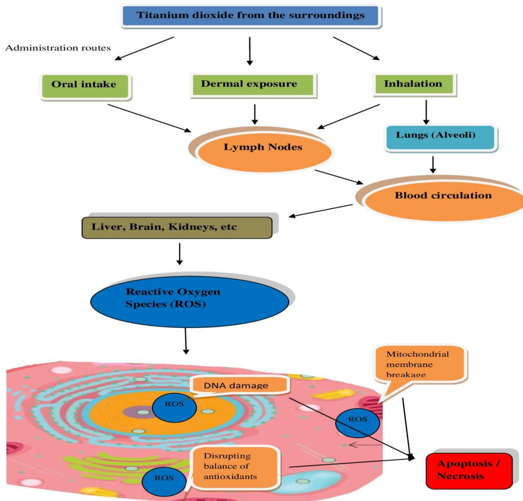
Fig. 1. Mechanism of toxicity induction and cell death by TiO 2 nanoparticles absorption
