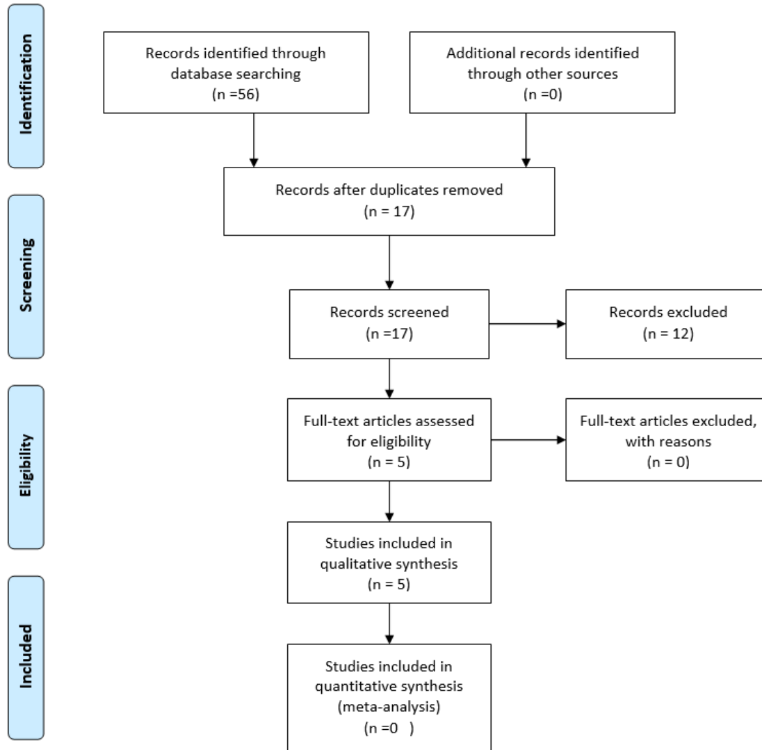
Fig.1: PRISMA flowchart.
