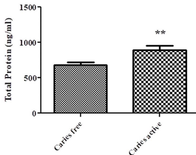
Fig 2. Comparison of salivary total protein concentration between Caries active (CA) and Caries free (CF) children. Values are represented as Mean \pm SEM. * significantly different compared to the CF group ( P < 0.01 ).
