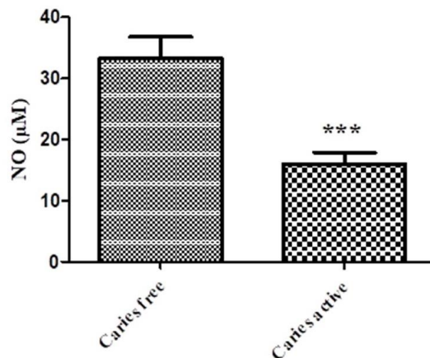
Fig 4. Comparison of salivary nitric oxide levels between Caries active (CA) and Caries free (CF) children. Values are represented as Mean \pm SEM. ***significantly different compared to the CF group ( P < 0.001 ).
