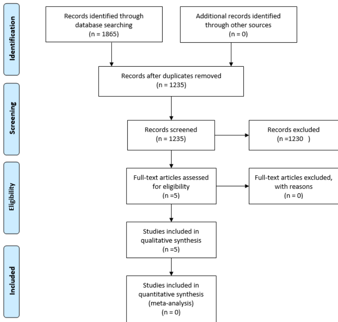
Fig.1: PRISMA flowchart.
