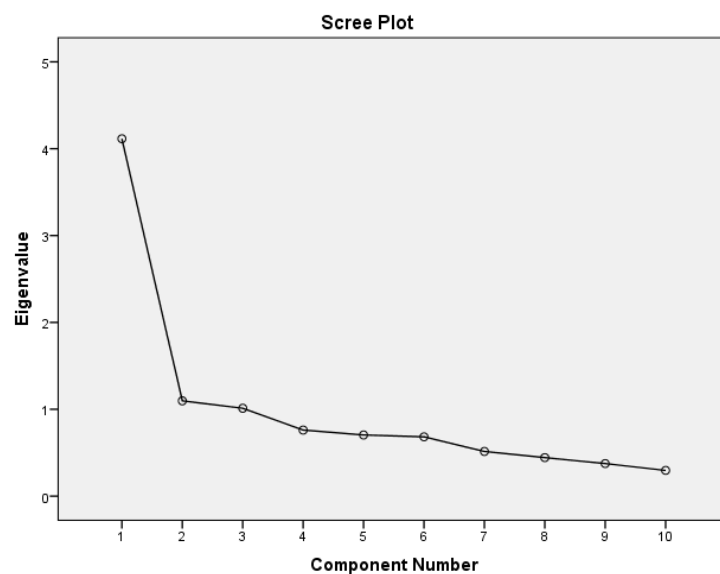
Fig. 1: Screen plot used for determining the number of factors (total items=10).
