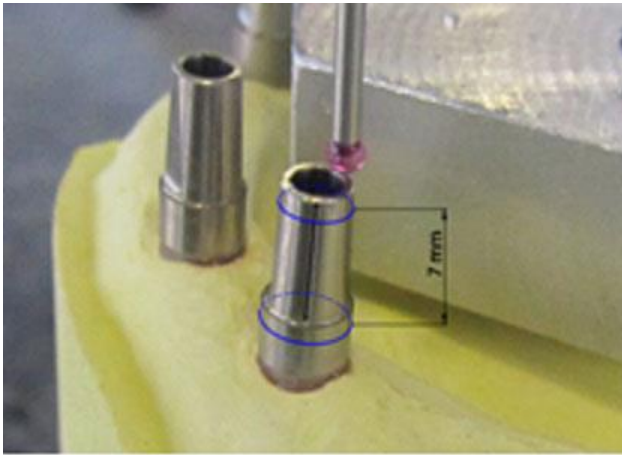
Fig. 5: Measurement of abutment direction (vertical and horizontal angles)
