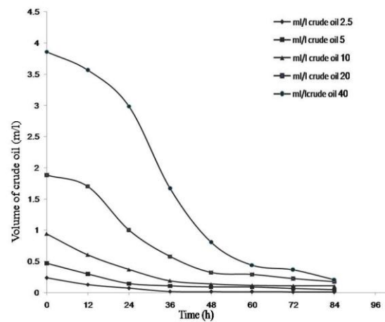
Fig. 3: Biodegradation curve at different initial crude oil concentrations
