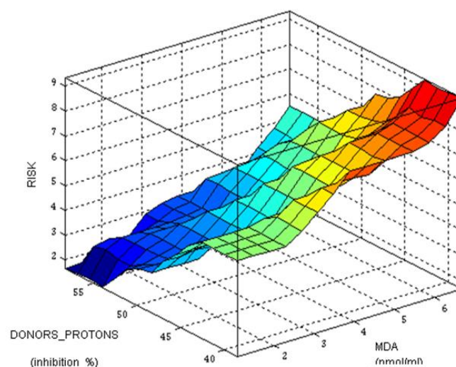
Fig. 4: Variation surface of the RISK
