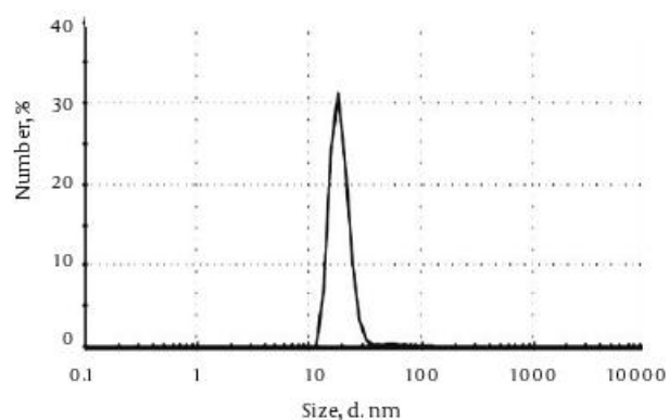
Figure 4. Particle Size Distribution of Colloidal Silver Nanoparticles
