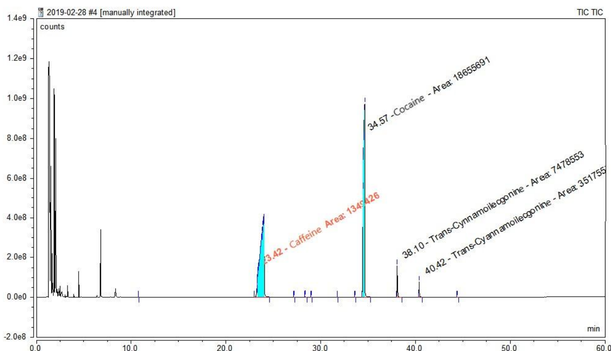
Figure 1. Analysis of the powder substance by gas chromatography mass spectrometry (GC-MS). The compound identification was achieved by quering and comparing the mass spectrum obtained (EI mass spectra, MS/MS spectra, and GC data with retention index) with reference mass spectra reported by NIST/EPA/NIH version 11. Caffeine and cocaine were the products obtained and both are marked in blue.
