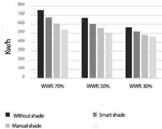
Fig. 14 Cooling load for the interior spaces during a year
