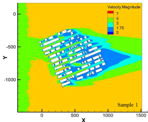
Fig. 10 Contour of absolute wind speed in meters per second, at 10 m balance; wind direction: west www.SID.ir
