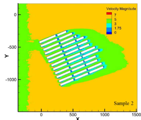
Fig. 10 Contour of absolute wind speed in meters per second, at 10 m balance; wind direction: west www.SID.ir
