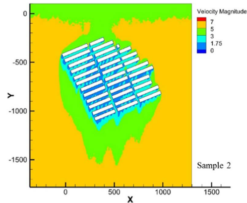
Fig. 9 Contour of absolute wind speed in meters per second, at 10 m balance; wind direction: north
