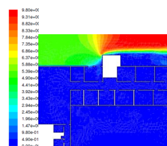
Fig. 6 Contours of velocity magnitude around the school (aisle window: close)
