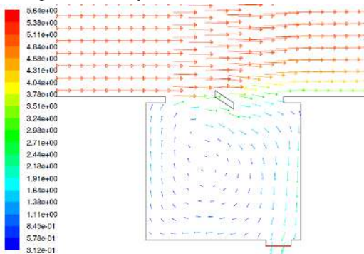
Fig. 18 Velocity vectors in 7th intervention, B (the door is open)
