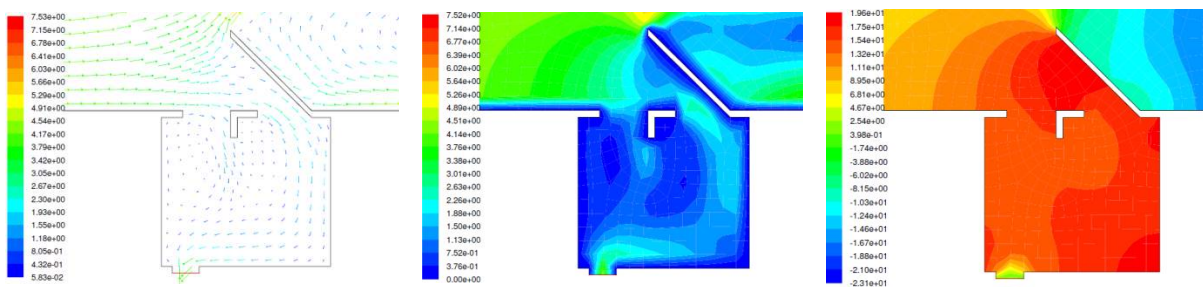
Velocity vectors Fig. 21 Contours of velocity magnitude and velocity vectors in 2th composed intervention.
