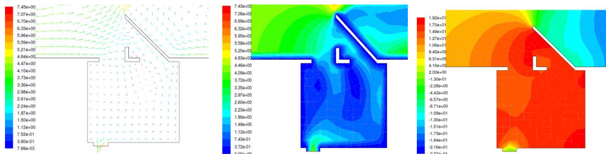
Velocity vectors Fig. 20 Contours of velocity magnitude and velocity vectors in 1th composed intervention
