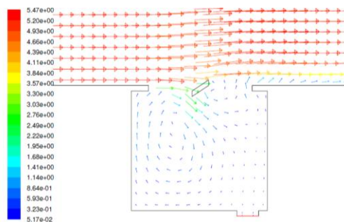
Fig. 17 Velocity vectors in 7th intervention
