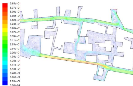
Fig. 5 Velocity vectors around the school
