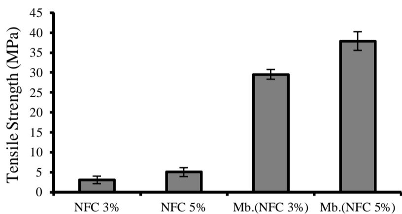
Fig. 8 Comparison tensile strength of nanocomposites with and without masterbatch (NFC: nanocellulose, Mb: masterbatch)
