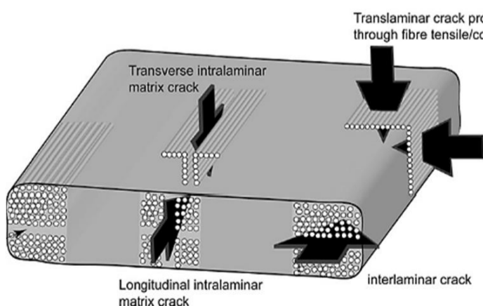
Fig. 4 Failure modes of composite materials [18]
