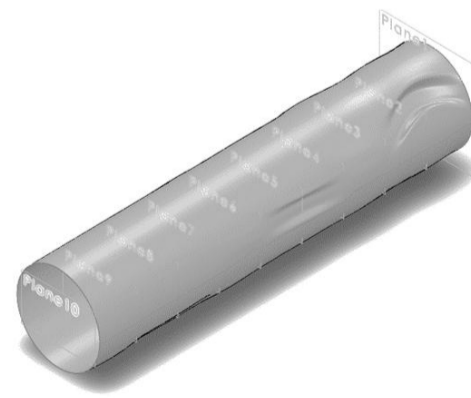
Fig. 9 Modeled pipe by gathered data through measuring device in SOLIDWORKS within coded APIs
