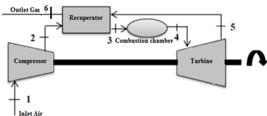
Fig. 1 Schematic of recuperated microturbine cycle
