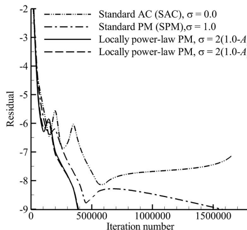
Fig. 18 Effect of the locally power-law PM on convergence rate around the NACA0012 hydrofoil at Re = 1100 , \alpha = 15^\circ
