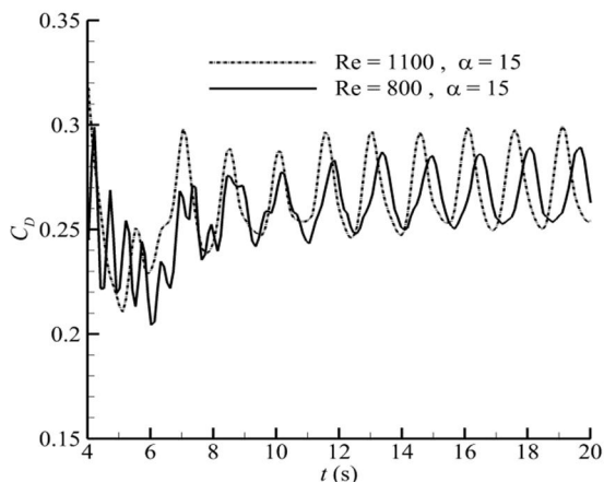
Fig. 19 Drag coefficient of the NACA0012 hydrofoil as a function of time \alpha = 15^\circ Re = 1100 and \alpha = 15^\circ Re = 800
