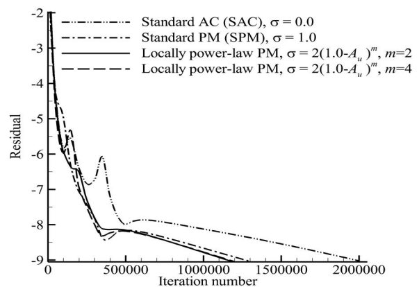
Fig. 14 Effect of the locally power-law PM on convergence rate around the NACA0012 hydrofoil at Re = 800 , \alpha = 20^\circ
