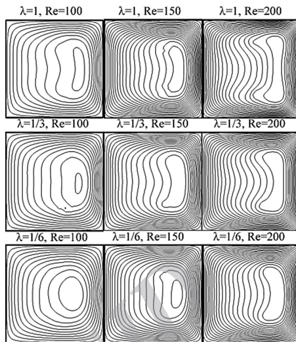
Fig.17 axial velocity contour for channels
