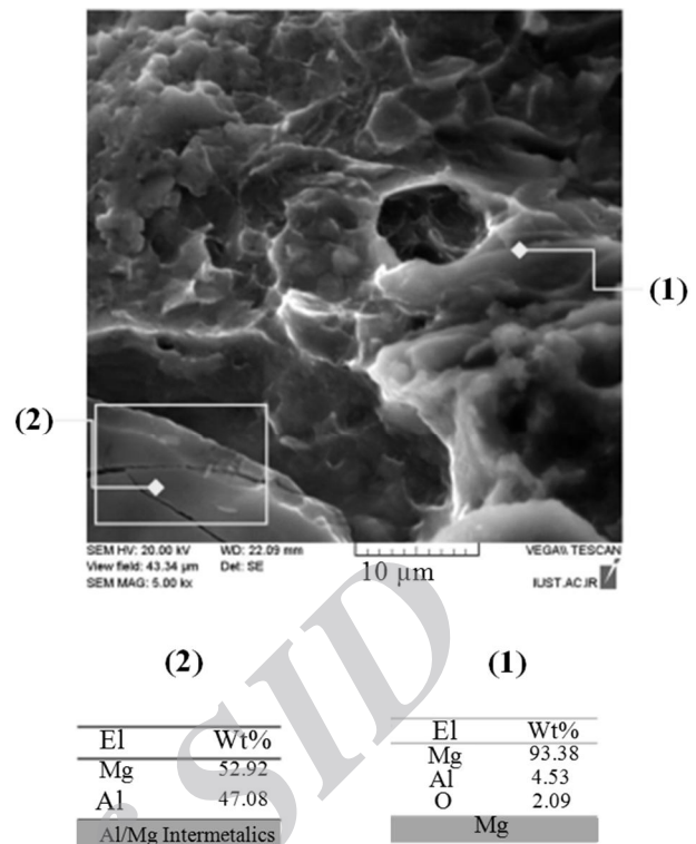
Fig. 16 SEM image of the fracture surface of magnesium in magnesium-top at high magnification
