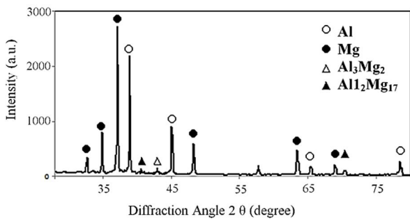
Fig. 18 XRD patterns of the in magnesium-top Retreading edge joint
