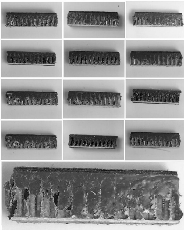
Fig. 15 Sections of flexible samples in the slot locations
