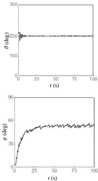
Fig. 13 Module positioning for \theta_i=200^\circ and \phi_i=60^\circ with 4 V activation voltage (a) \theta , (b) \phi
