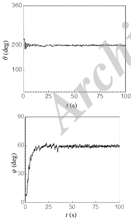
Fig. 15 Module positioning for \theta_i=200^\circ and \phi_i=60^\circ with 5 V activation voltage (a) \theta , (b) \phi
