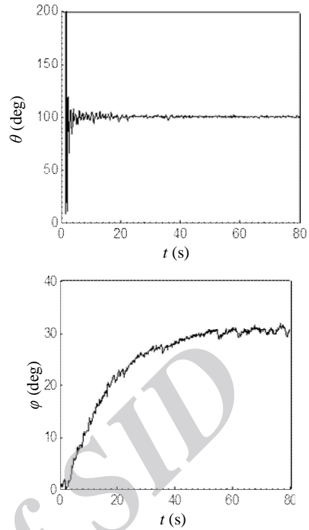
Fig. 12 Module positioning for \theta_i=100^\circ and \phi_i=30^\circ with 4 V activation voltage (a) \theta , (b) \phi
