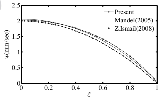
Fig. 2 Comparison of the axial velocity profile for non tapered artery with [16], [29]
