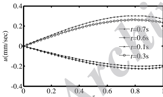
Fig. 4 Radial velocity profiles for different time
