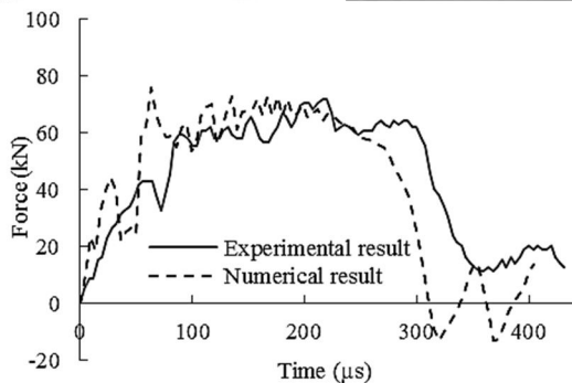
Fig. 19 Force-time curves and final shape of the tubes after deformation in both numerical and experimental models for v=89\text{m/s} , m=1775\text{gr}
