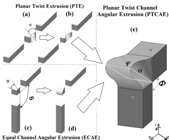
Fig. 3 Schematic of (a) bidirectional and (b) unidirectional planar twist extrusion processes, equal channel angular extrusion with (c) variable \Phi and \Psi and (d) -\Psi = \Phi and (e) planar twist channel angular extrusion
