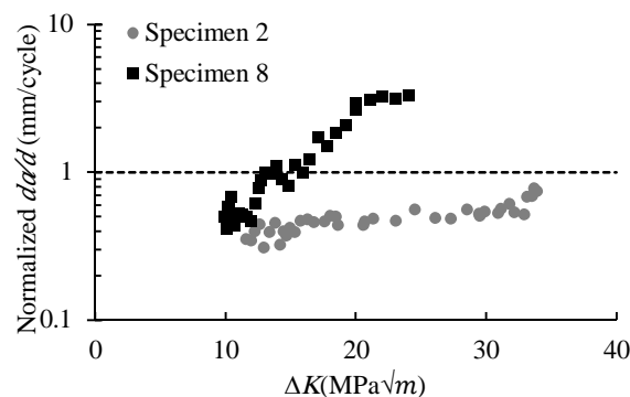
Fig. 10 Effect of rotational speed on normalized crack growth rate at traverse speed of 16 mm/min
