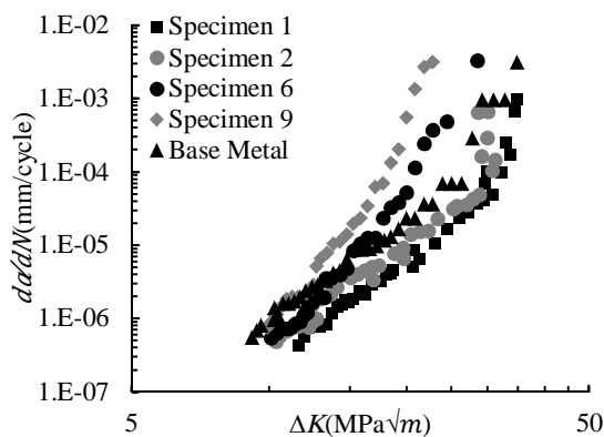
Fig. 7 Experimental fatigue crack growth vs. stress intensity factor range of base metal and some welded specimens
