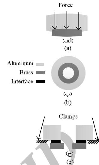
Fig. 5 Schematic of the samples were prepared for Chalmers test; (a) general scheme and direction of applied force, (b) top view, (c) cross-section view
