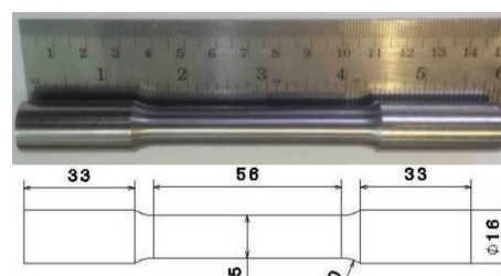
Fig. 13 The specimen used for the tension test
