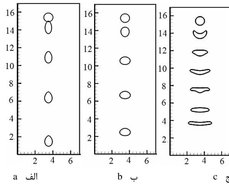
Fig. 21 Shape evolution of ferrofluid droplet for different Eo numbers (a: Eo=3, b: Eo=10 and c: Eo=20) at Oh=0.08, Bo_m=9.6 and \chi=2 in a vertical magnetic field
