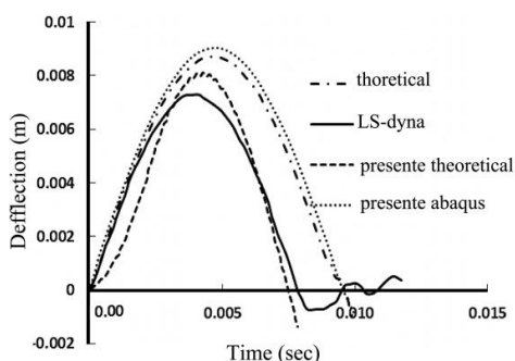
Fig. 4 The deflection of the top face beam at impact from Finite element analysis and analytical
