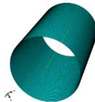
Fig. 15 Meshing of aluminium tube in ABAQUS software
