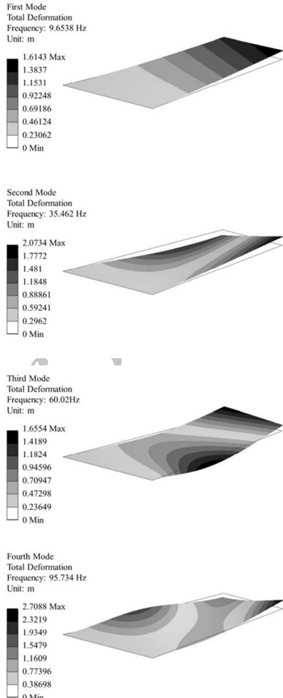
Fig. 5 Modal analysis mode shapes
