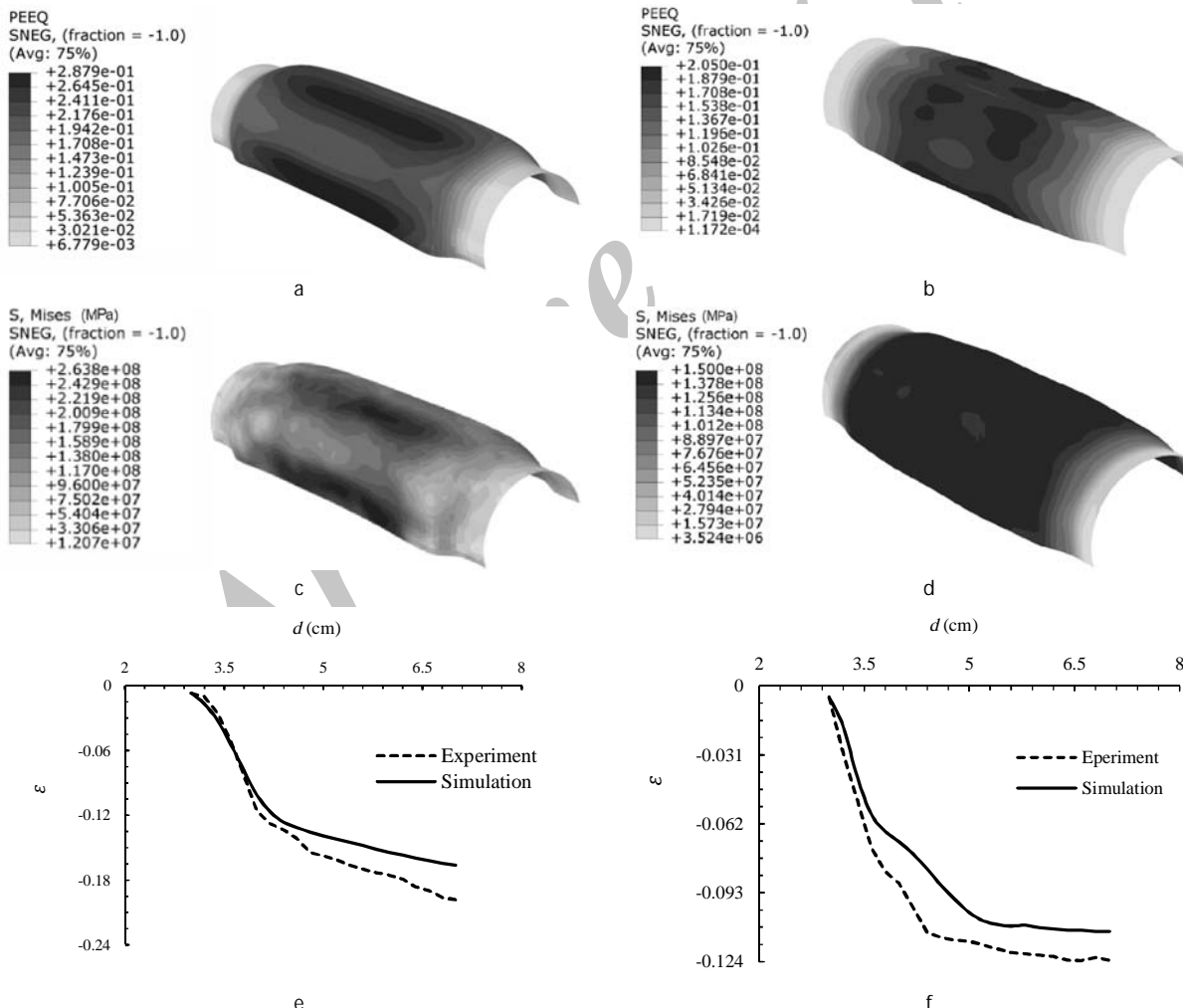
Fig. 18 (a) Equivalent plastic strain for rectangular sample, (b) Equivalent plastic strain for bulged sample, (c) Mises stress distribution for rectangular sample, (d) Mises stress distribution for bulged sample, (e) Thickness strain for rectangular sample along path b, (f) Thickness strain for bulged sample along path a
