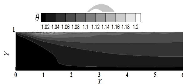
Fig. 5 Temperature distribution in the air flow cavity for air mixture with 10% \text{CO}_2 and 20% \text{H}_2\text{O} , RC=10
