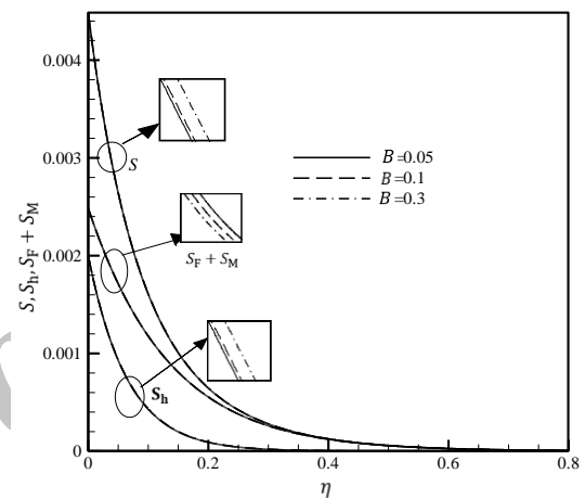
Fig.9 (a,b). Effect of B parameter on Be, F'(\eta), F''(\eta), \theta(\eta), \theta'(\eta), S, S_h and S_F + S_M in su=3, Pr=2.4, a=1, n=2, M^2 = 2 شکل 9- الف، ب اثر پارامتر B بر Be, F'(\eta), F''(\eta), \theta(\eta), \theta'(\eta), S, S_h و S_F + S_M در M^2 = 2, n=2, a=1, Pr=2.4, su=3
