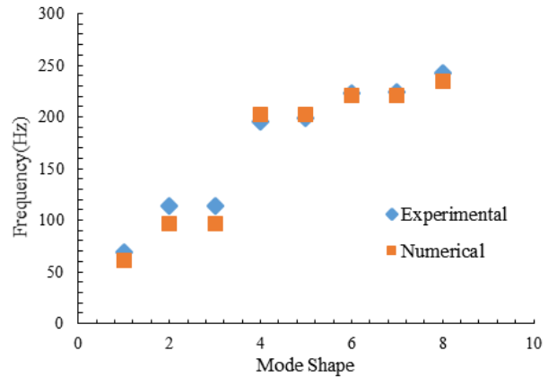
Fig. 18 Comparison of numerical results with the experimental results of Re. [12] for the first eight frequencies tire model
