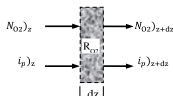
Fig 2 Control volume in the cathode catalyst layer
