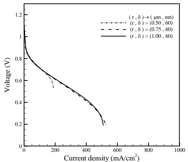
Fig 13 Effect of agglomerate radius on performance curve
