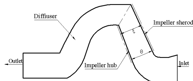
Fig. 2 Meridional view of one stage of pump
