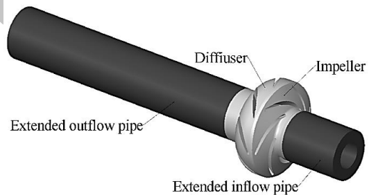
Fig. 3 Geometry of pump model used in simulation
