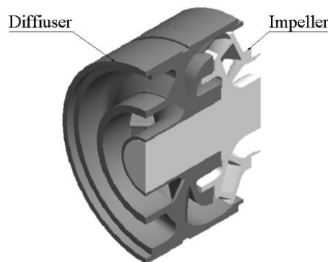
Fig. 1 3D geometry of one stage of pump modeled in Solid work
